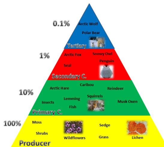
Arctic Tundra Energy Pyramid
